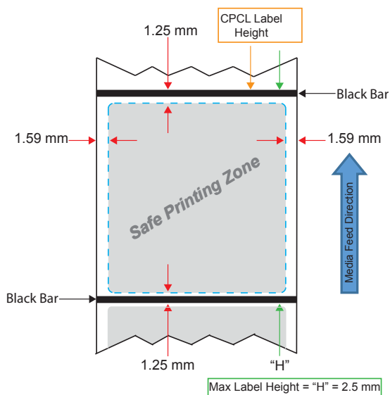
Figure 23 • Black Bar Label Media
