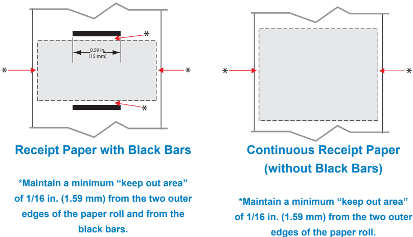
Figure 26 • Keep Out Areas
