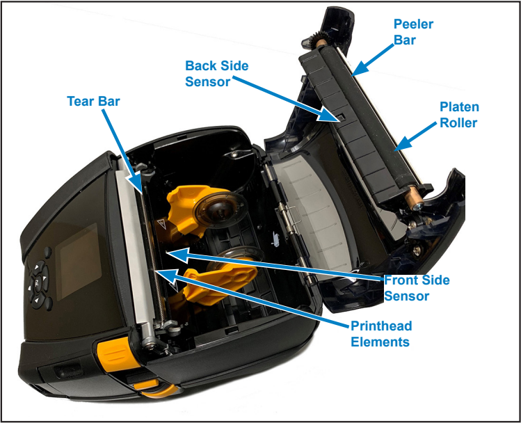
Figure 32 • ZQ630 Cleaning (Linered)
