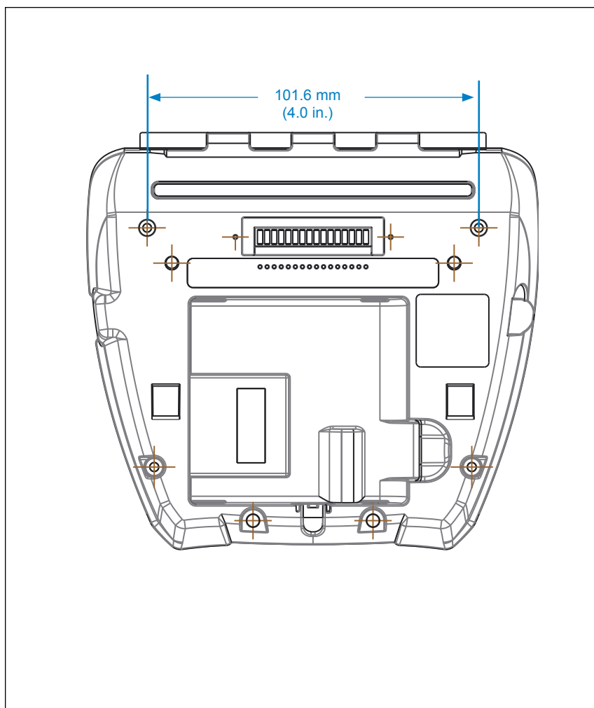
Figure 38 • ZQ630 Mounting Hole Dimensions
